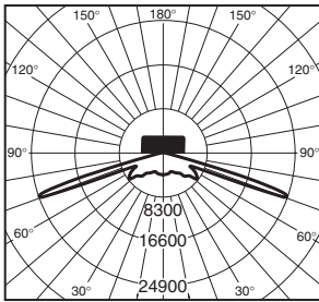
Typical Candlepower Distribution of 400W MH Parking/Roadway Light. (Front View)
