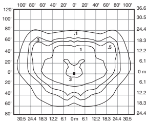
Isofootcandle plot of one 400W MH Parking/Roadway Light at 30' (9.1 m) mounting height, and 0° tilt above horizontal.
